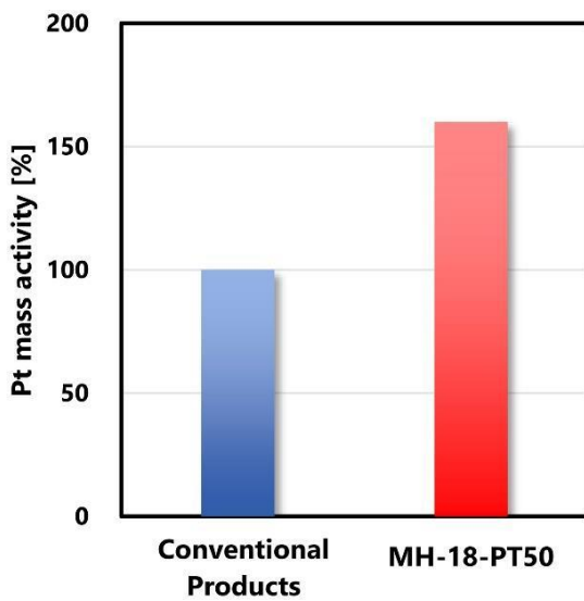
Fig.4 Catalytic activity performance in fuel cells (Source: N.E. CHEMCHAT)
